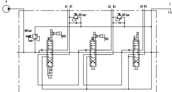
HYDRAULIC CIRCUIT
