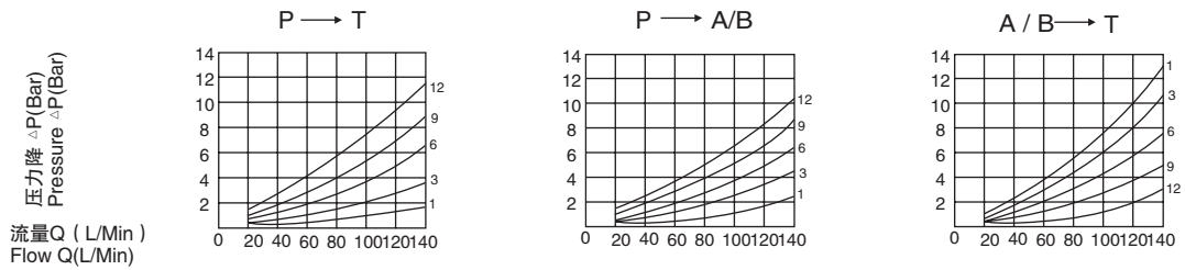
压力损失曲线 Pressure Drop Flow Curves
