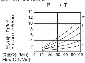
压力损失曲线 Pressure Drop Flow Curves
